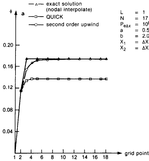
FIG. 4a. Numerical solutions to test problem II (downstream boundary condition: d\phi/dx=0 ). Starting calculation method: \phi_1 = \phi(0) = 0 , \phi_2 by first-order upwind.
