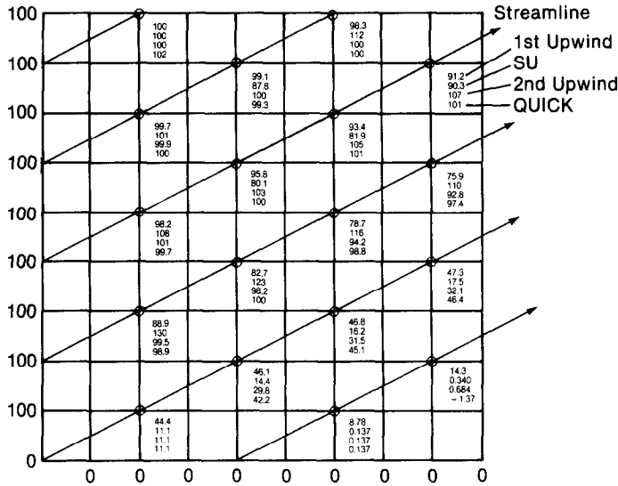
FIG. 7. Numerical solutions to Eq. (18) (upstream boundary conditions: \phi(0, y) = 100, 0 < y \leq 1, \phi(x, 0) = 0, 0 \leq x \leq 1 ).
